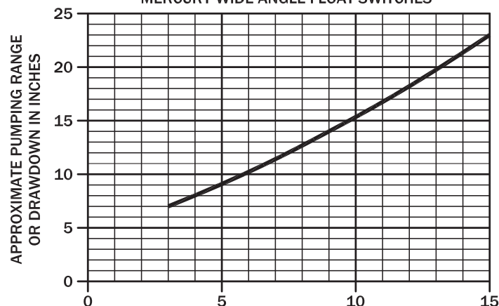
TETHER LENGTH VS. DRAWDOWN FOR MERCURY WIDE ANGLE FLOAT SWITCHES
