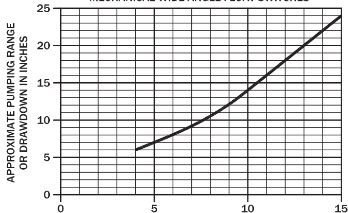
TETHER LENGTH VS. DRAWDOWN FOR MECHANICAL WIDE ANGLE FLOAT SWITCHES
